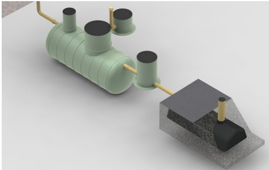
Biocleaner with tunnels
