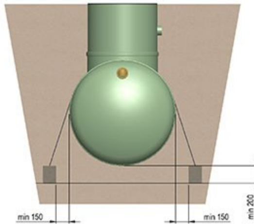
Installation with sleepers
