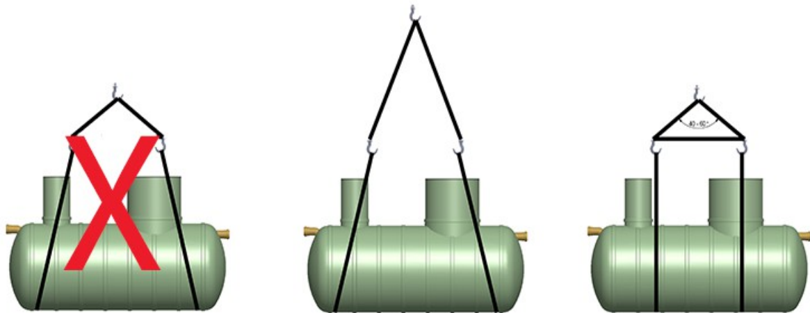
Lifting
