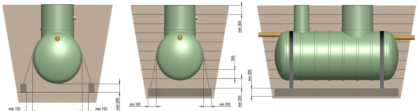
Anchoring
