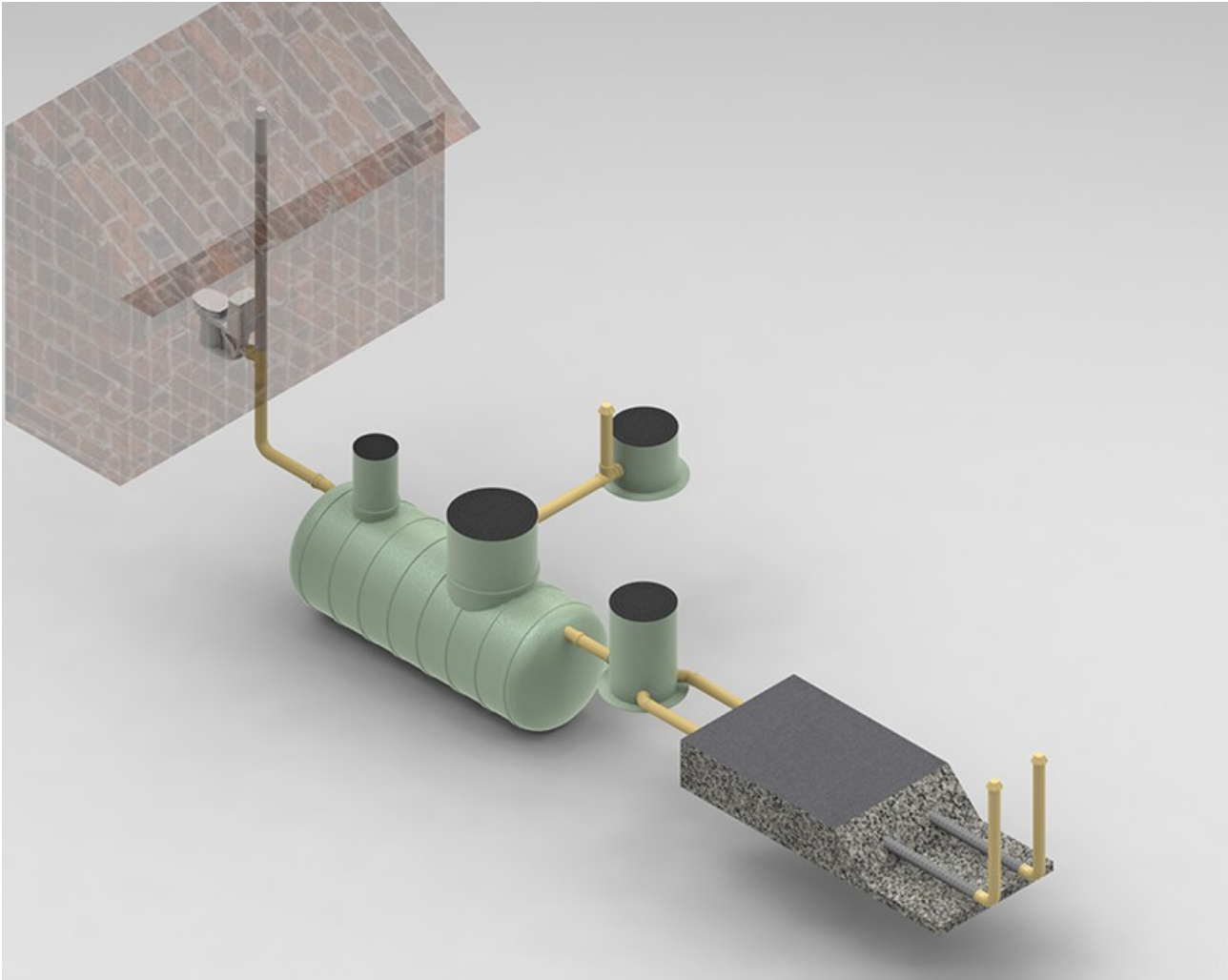
Infiltration field
