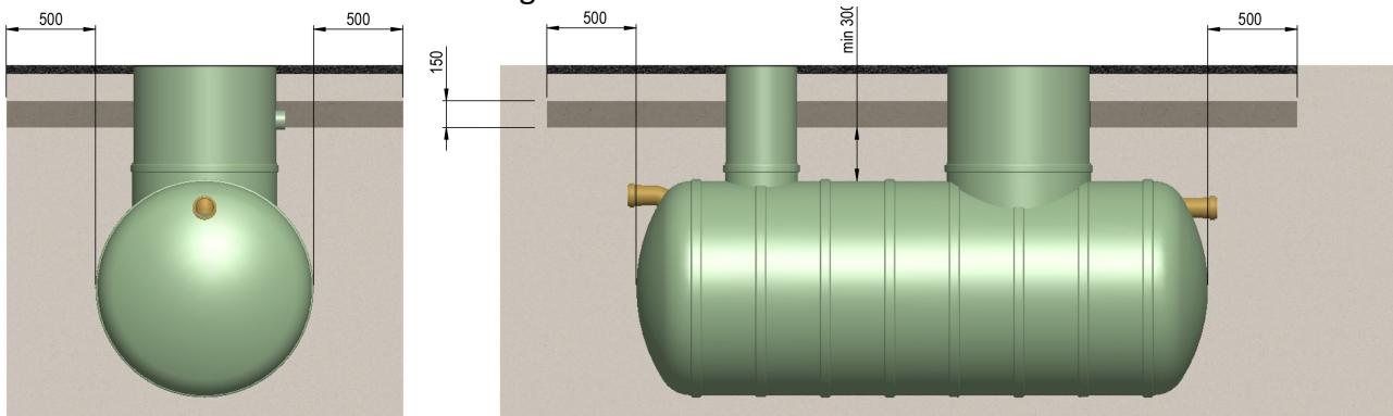
Traffic load installation
